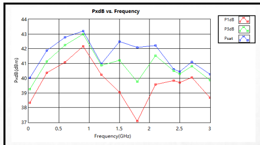
PndB vs. Frequency CW
