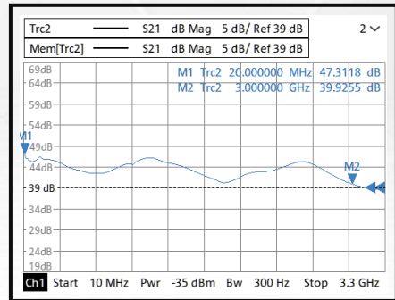
Gain@-40°C
