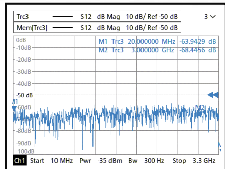
Isolation@-40°C
