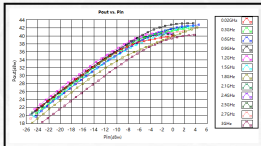
Pout vs. Pin CW
