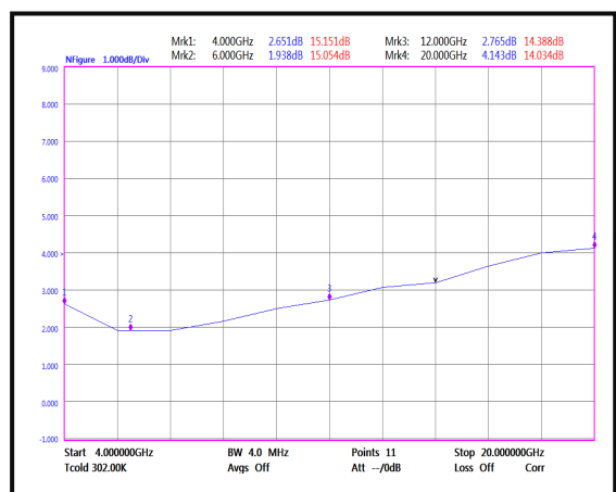
Noise Figure (4GHz-20GHz)
