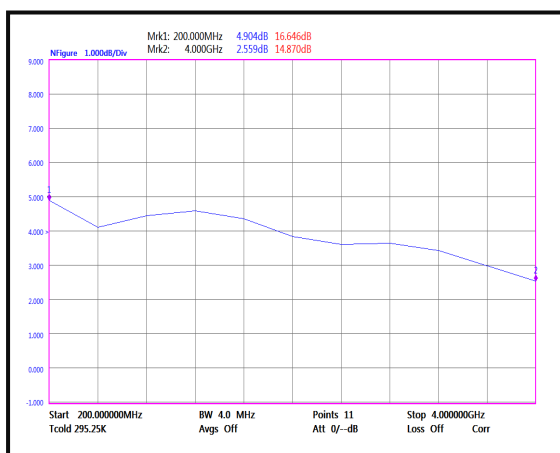
Noise Figure (200MHz-4GHz)
