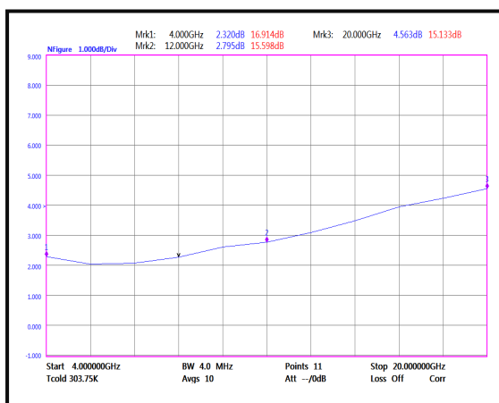
Noise Figure(4-20GHz)
