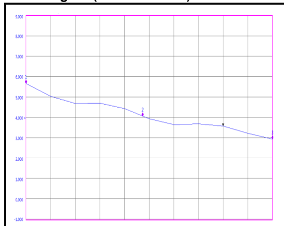
Noise Figure (200MHz-4GHz)
