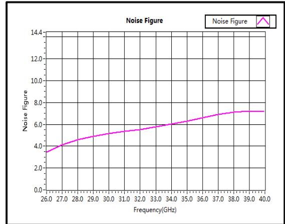
Noise Figure (26-40GHz)
