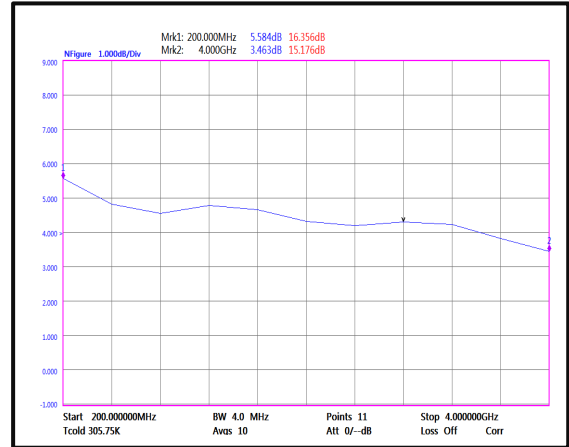
Noise Figure (0.2-4GHz)
