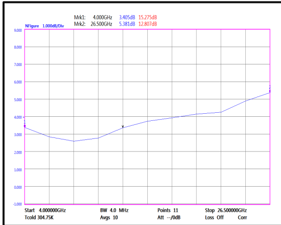
Noise Figure (4-26.5GHz)
