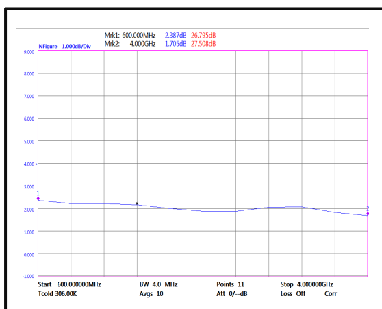
Noise Figure (600MHz-4GHz)
