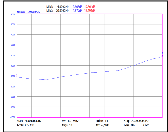
Noise Figure(4GHz-20GHz)
