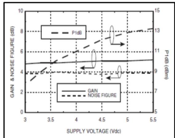
Gain, Noise Figure & P1dB vs. Supply Voltage 500 MHz
