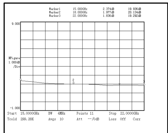
Noise Figure
