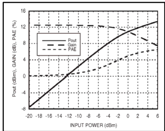
Power Compression @25GHz
