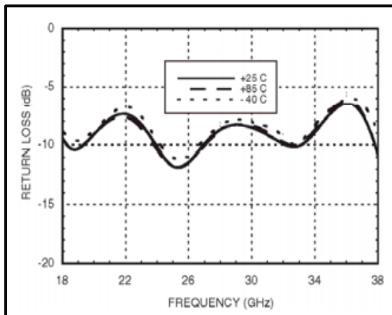
Output Return Loss vs. Temperature
