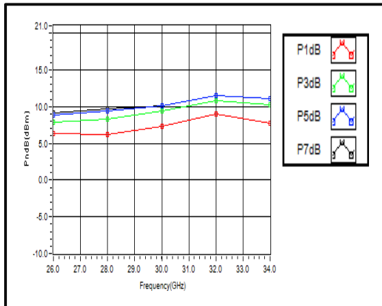
PxdB vs. Frequency (Vcc= +3V)
