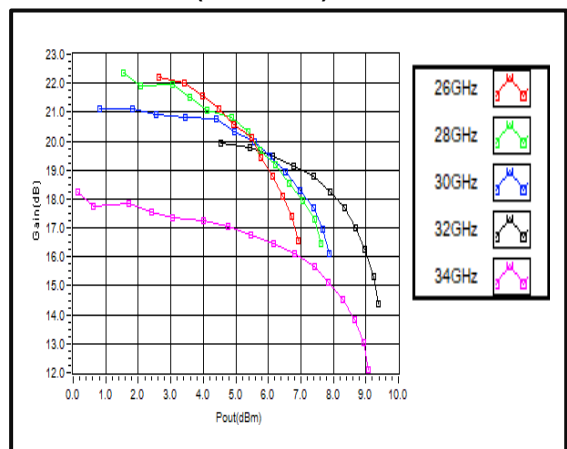
Gain vs. Pout (Vcc= +2V)
