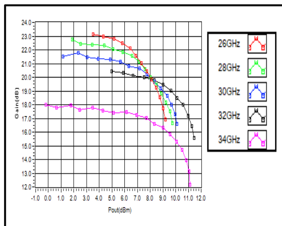
Gain vs. Pout (Vcc= +3V)
