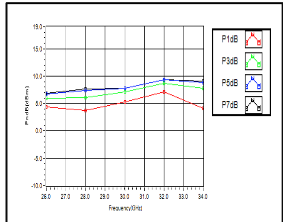
PxdB vs. Frequency (VCC= +2V)
