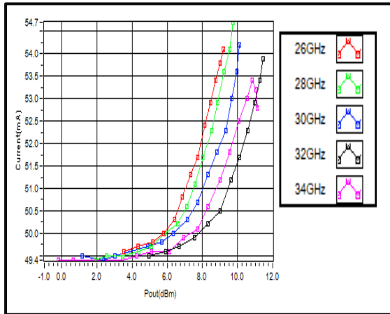
Current vs. Pout (Vcc= +3V)
