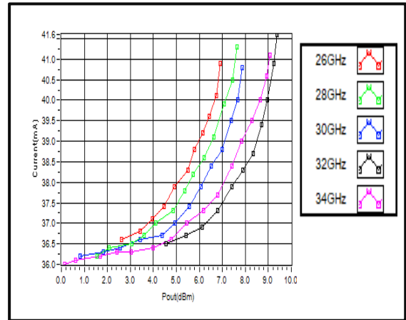
Current vs. Pout (Vcc= +2V)
