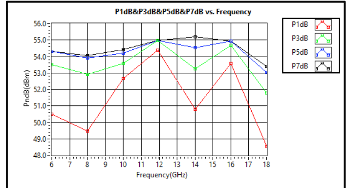
PxdB vs Frequency *Pulse With default 20dB Attenuation
