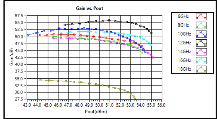
Gain vs Output Power *Pulse With default 20dB Attenuation
