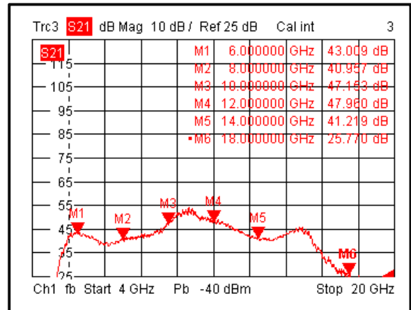
Gain vs. Frequency @+25°C With 30dB Attenuation
