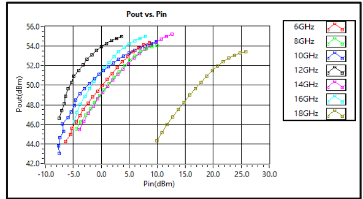
Output vs Input Power *Pulse With default 20dB Attenuation
