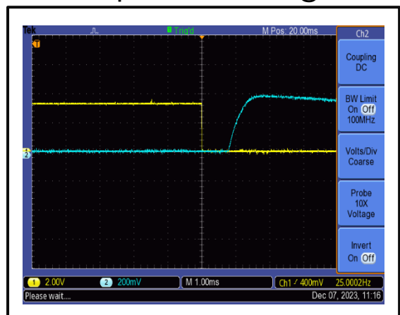
The Gates Open Time is 1500 us @+25°C
