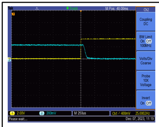
The Drains Closure Time is 200 us @+25°C
